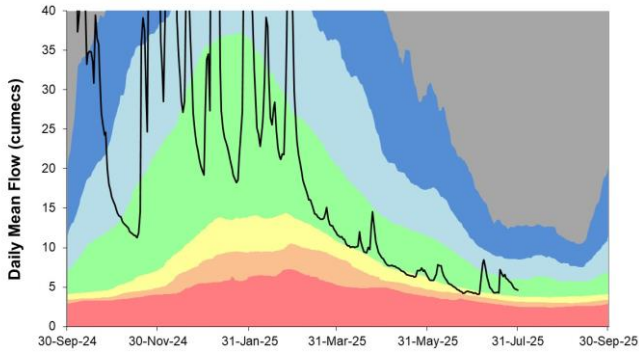
Offord (Gross flows), GREAT OUSE
