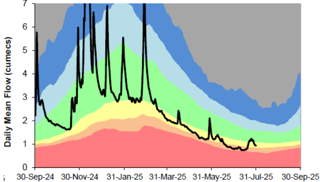
Swanton Morley Total Flow, Wensum
