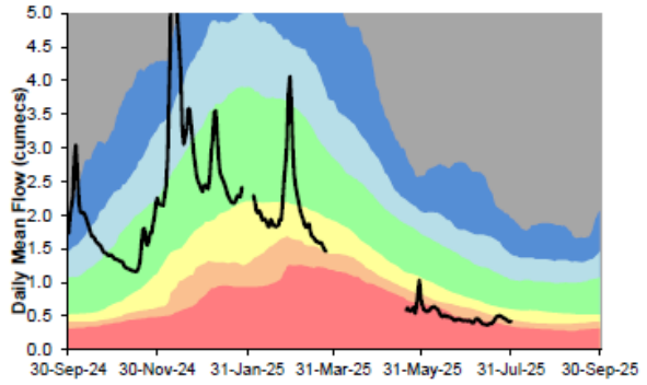
SPRINGFIELD, River Chelmer
