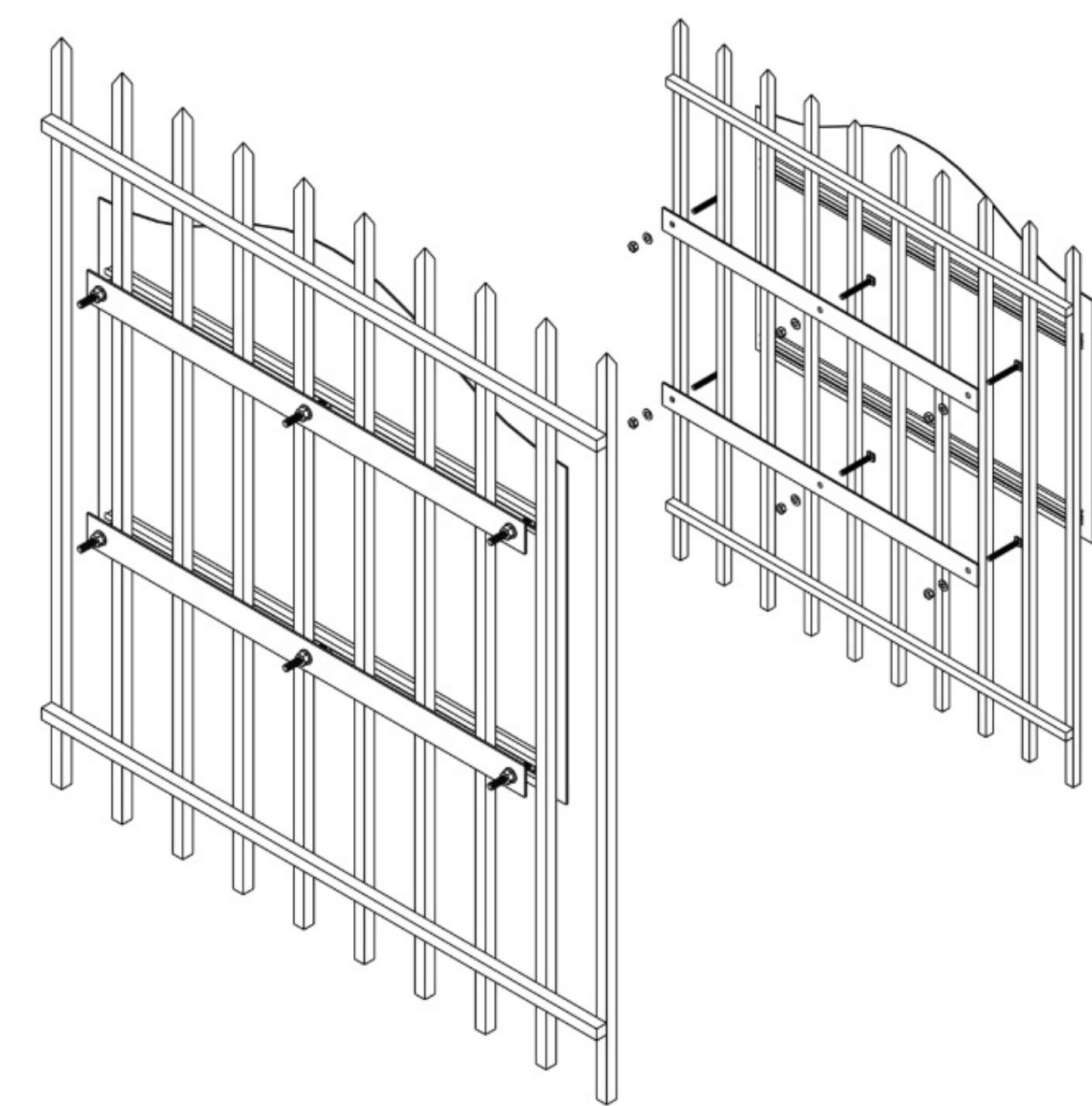
Fence fixing kit example
