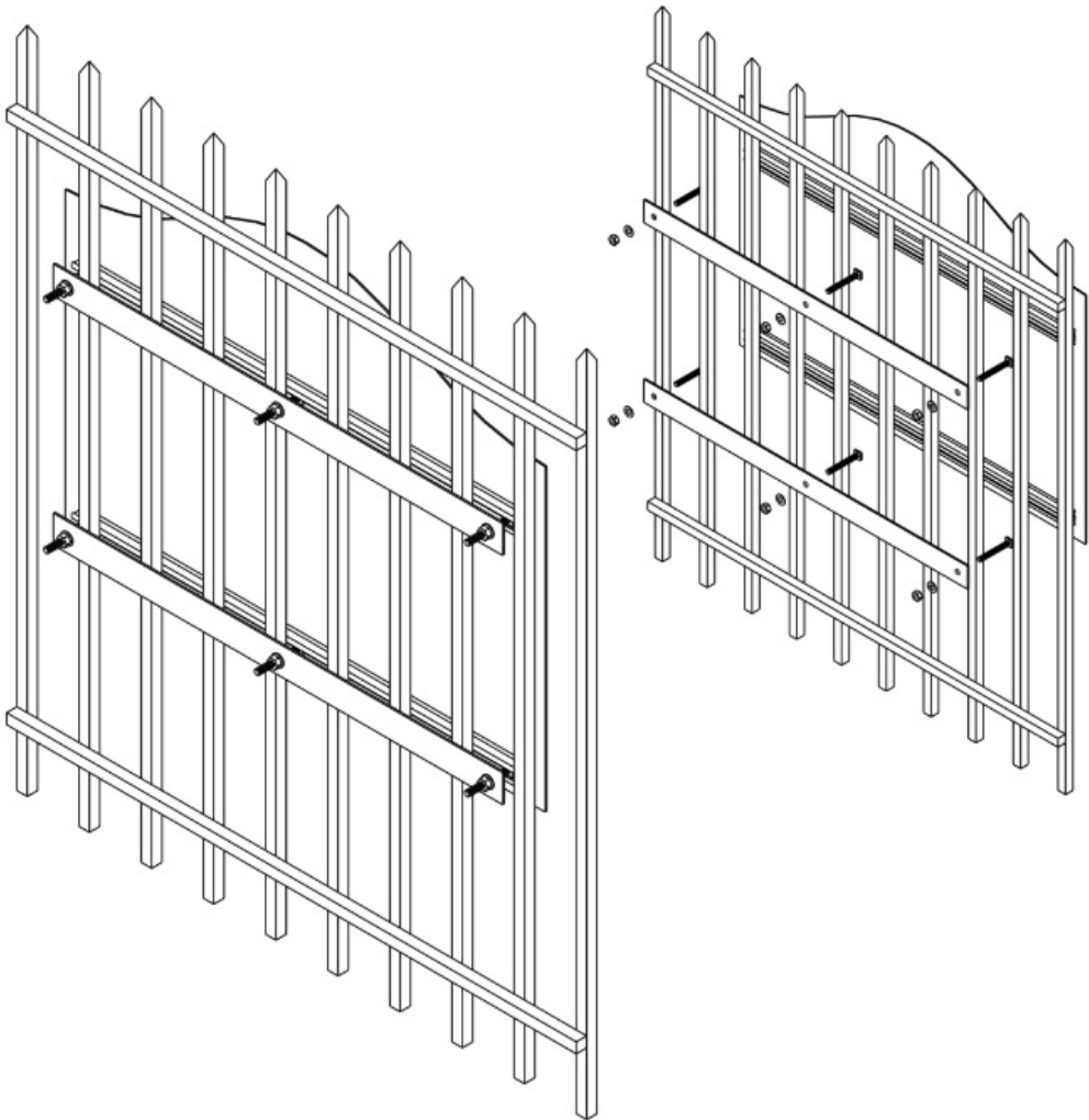
Fence fixing kit example
